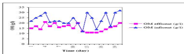
Figure 5. Organic matters before and after treatment in digester [29].
