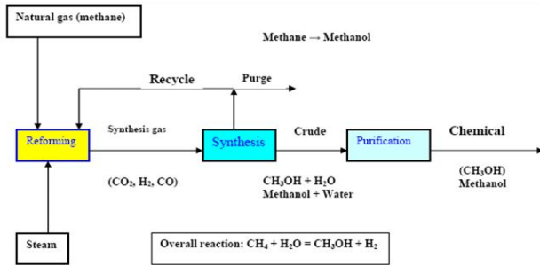
Figure 2. Schematic diagram shows methanol production [16].
