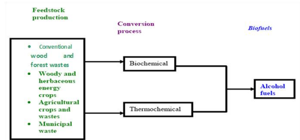
Figure 8. Biofuel pathways for renewable alcohol fuels [30].
