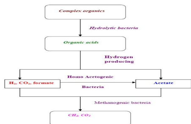
Figure 3. Biogas production process [26].
