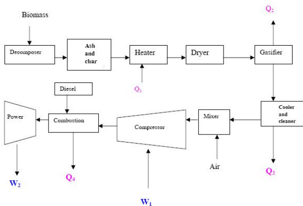
Figure 7. Advanced biomass power with diesel engine [30].
