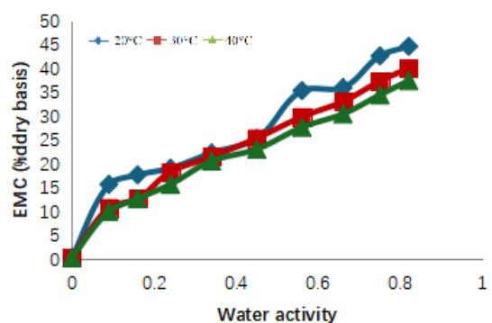
Figure 11. Effect of Water Activity on Equilibrium Moisture Content of Ighu from NR 8082 (Udi Method).
